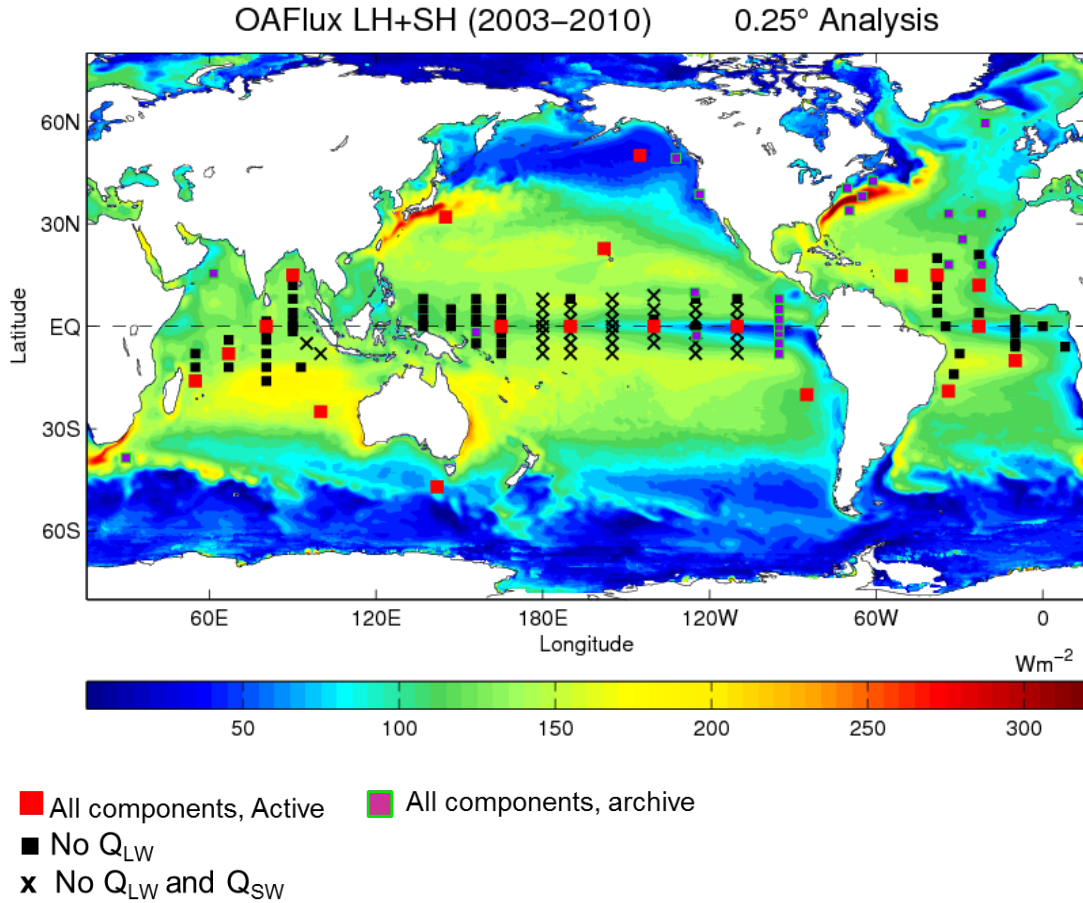
Fig. 6. Moored buoy locations over the global oceans superimposed onto the 0.25-degree OAFlex analysis of surface latent and sensible heat fluxes (colored background). Red squares denote full-flux buoy sites that provide all flux components (shortwave, longwave, latent and sensible heat fluxes, winds). Black squares denote the buoy sites that provide all flux components except longwave radiation. Crosses denote the sites that provide air–sea variables and winds for computing latent and sensible heat fluxes and wind stress only (from Li.san Yu).
